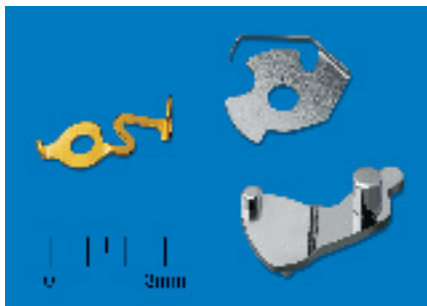
Etampes progressives
