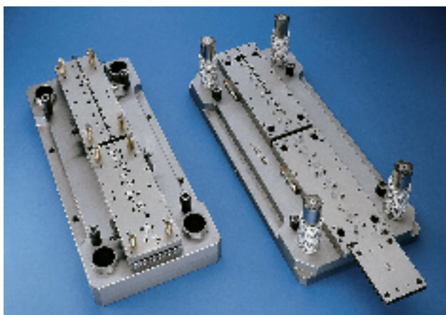
Etampes progressives
